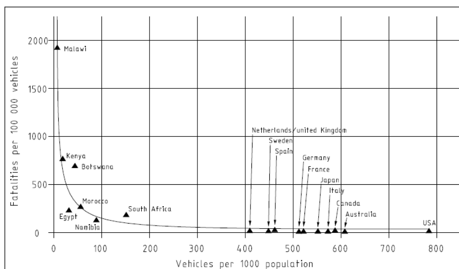
Figure 4.4 Fatalities per 1000 vehicles (SATCC, 2003)
